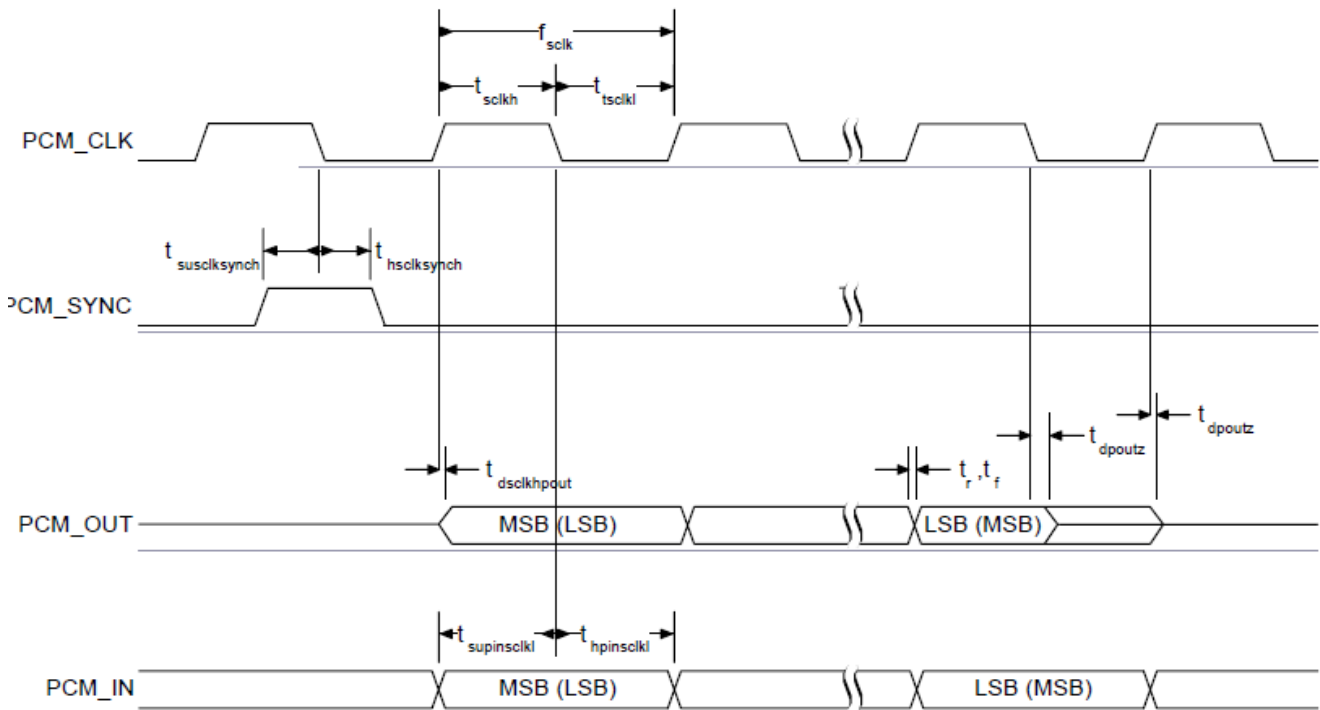
PCM Slave Timing Short Frame Sync
