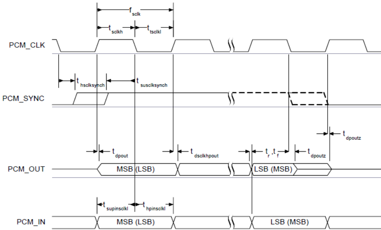
PCM Slave Timing Long Frame Sync
