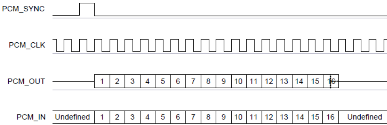
Short Frame Sync (Shown with 16-bit Sample)
