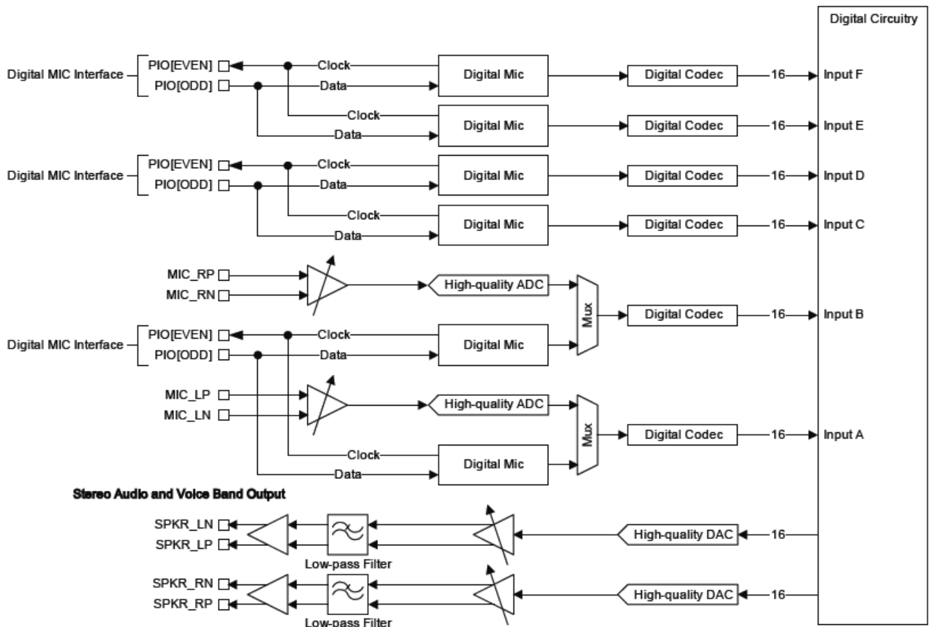
Stereo Codec Audio Input and Output Stages
