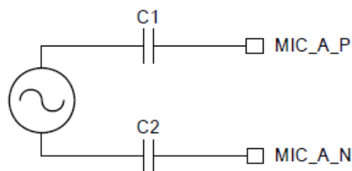
Differential Input (Single Channel Shown)
