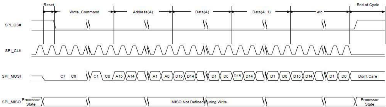
SPI Write Operation
