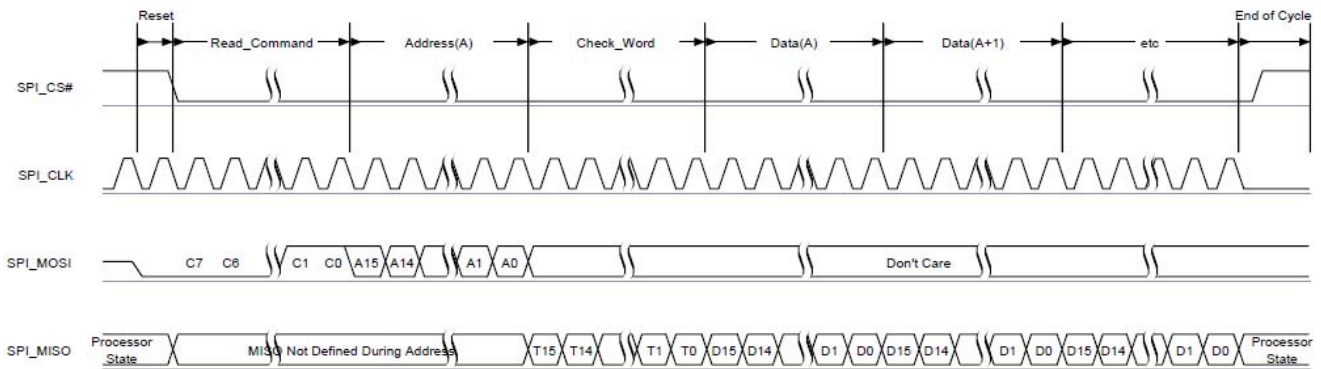
SPI Read Operation
