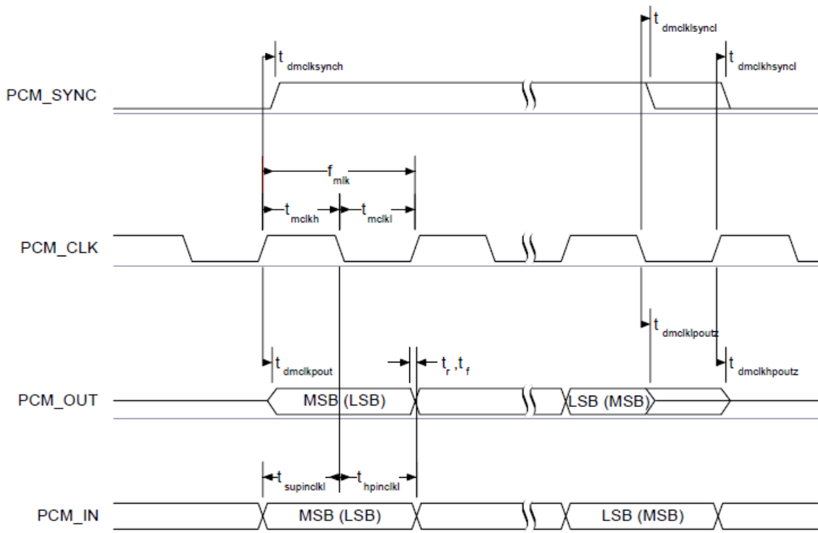
PCM Master Timing Long Frame Sync
